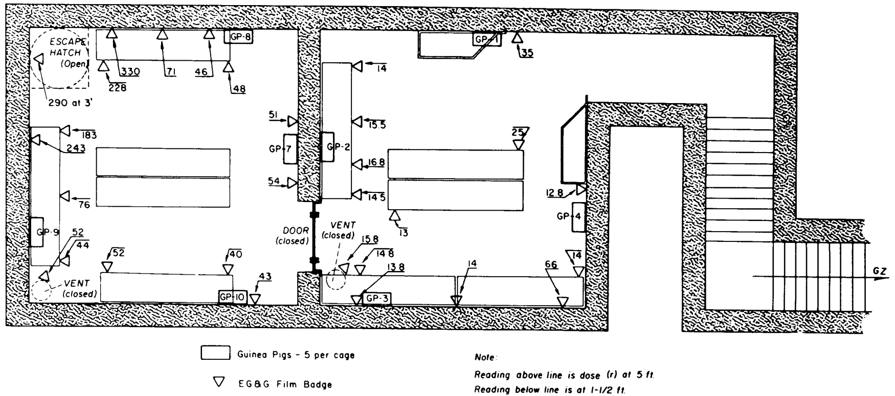
Fig. 6—Locations and types of measurements recorded by various radiation dosimeters inside shelter 8002.
